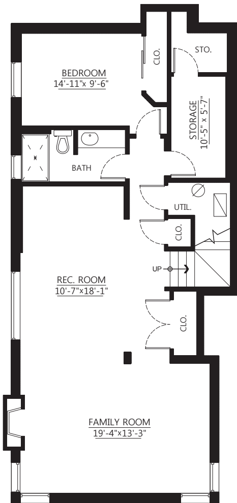
Lower Floor Plan Floor Area: 1,096 sq.ft.
